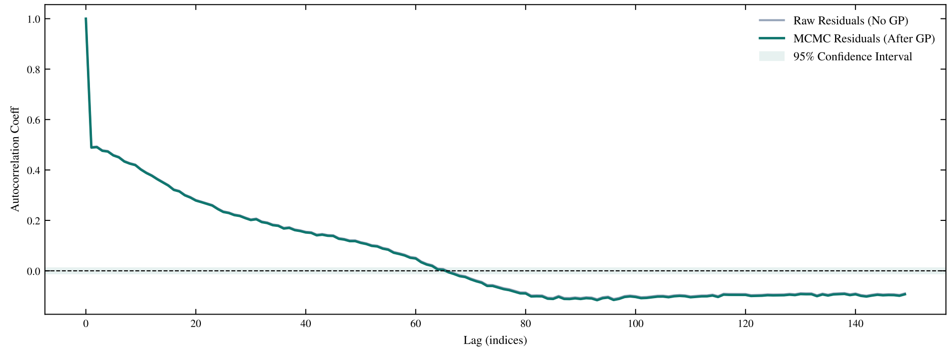
TIC 136274063 | Sectors: 102, 103 | GP Residuals Autocorrelation Function (ACF)
