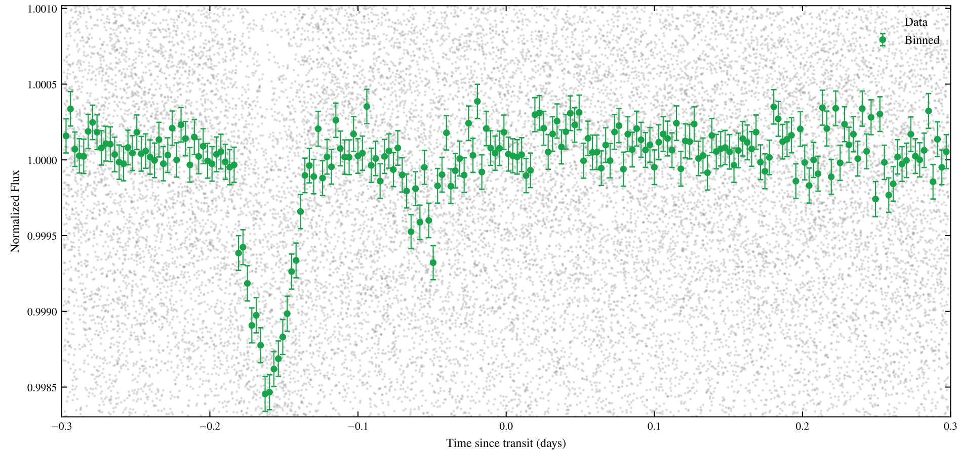
TIC 136274063 | Sectors: 102, 103 | Phase-Folded Transit (P = 0.59713 d)
