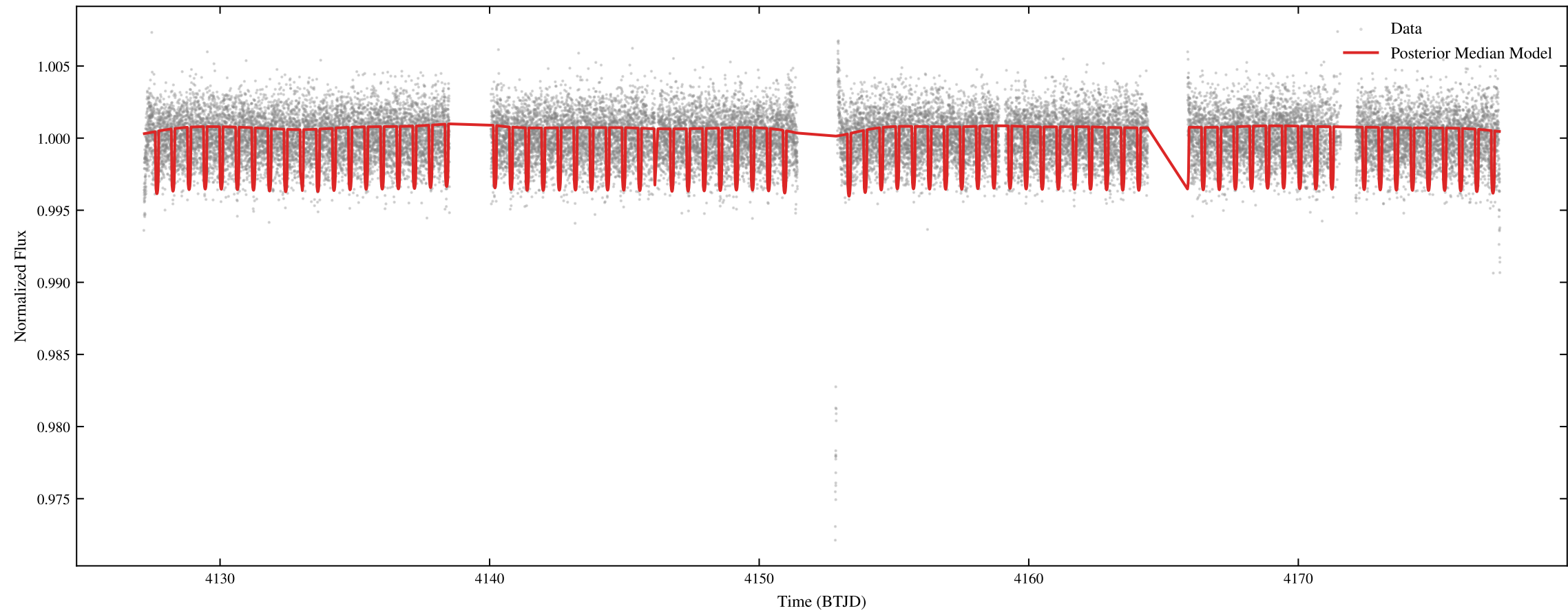
TIC 136274063 | Sectors: 102, 103 | MCMC Posterior Predictive Check
