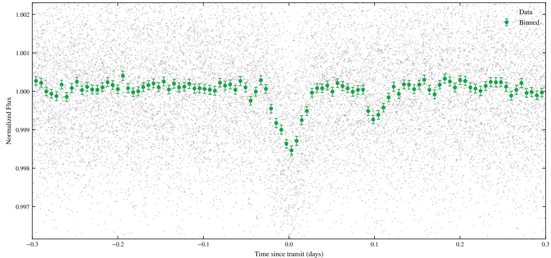
TIC 136274063 | Sectors: 102, 103 | Phase-Folded Transit (P = 1.19452 d)
